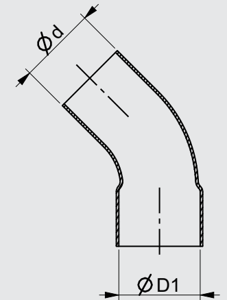
Part Drawing
